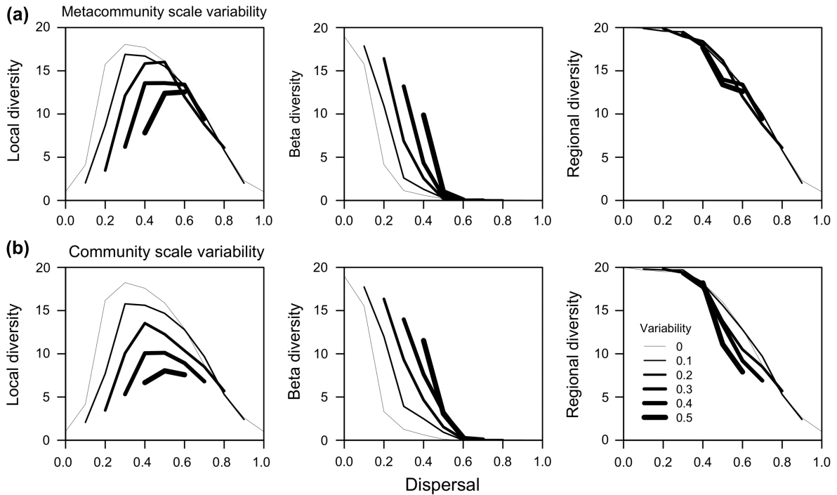
Figure 2. Local richness (alpha), spatial turnover (beta) and regional (gamma) species richness as function of dispersal (x axis) for two spatial scales of dispersal stochasticity – (a) metacommunity and (b) community levels; lines with increasing thickness indicate values of dispersal stochasticity (i.e. 0, 0.1, 0.2, 0.3, 0.4 and 0.5). We present means over 100 simulations (standard deviations are omitted for clarity but are always inferior to 2%). Predictions are only presented for scenarios where deviations from mean dispersal do not exceed realized dispersal of 0 or 1. For example, for a = 0.2 , values of dispersal stochasticity are only shown for a maximum dispersal stochasticity of 0.2 so that the range of dispersal values were between 0 and 0.4. This procedure avoided any potential border effect (see Methods section for details).
